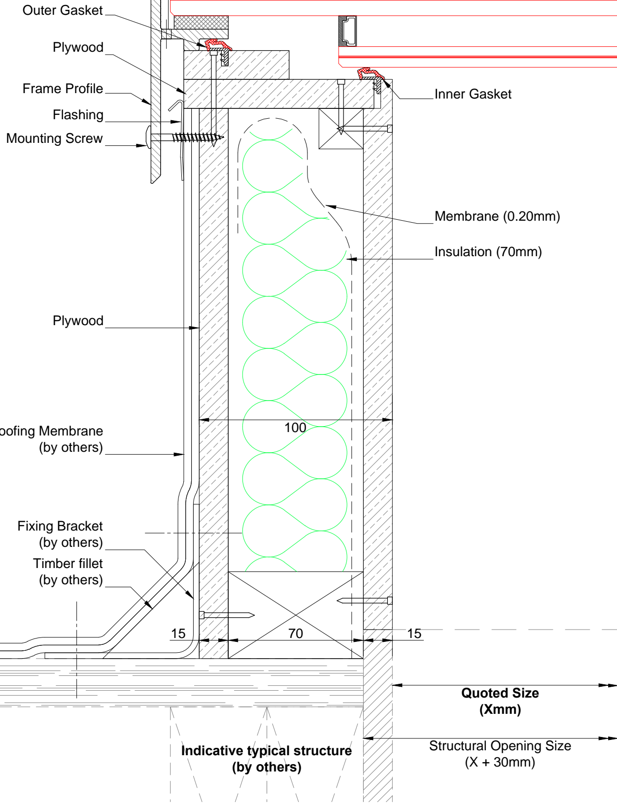
SCALE 1:2 @ A3
